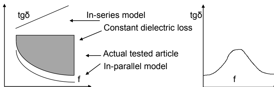
Low frequency dielectric loss curve (<1kHz)
